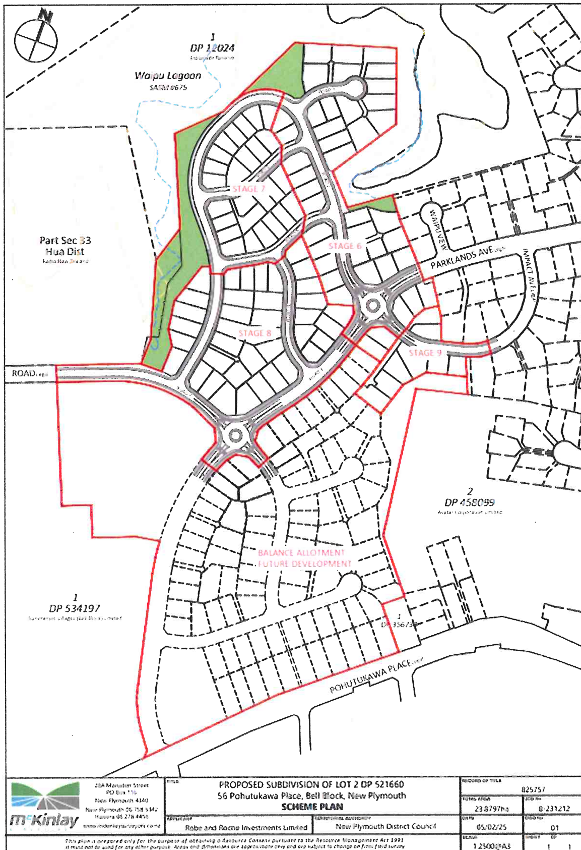
Figure 1 – McKinlay Surveyors Scheme Plan
