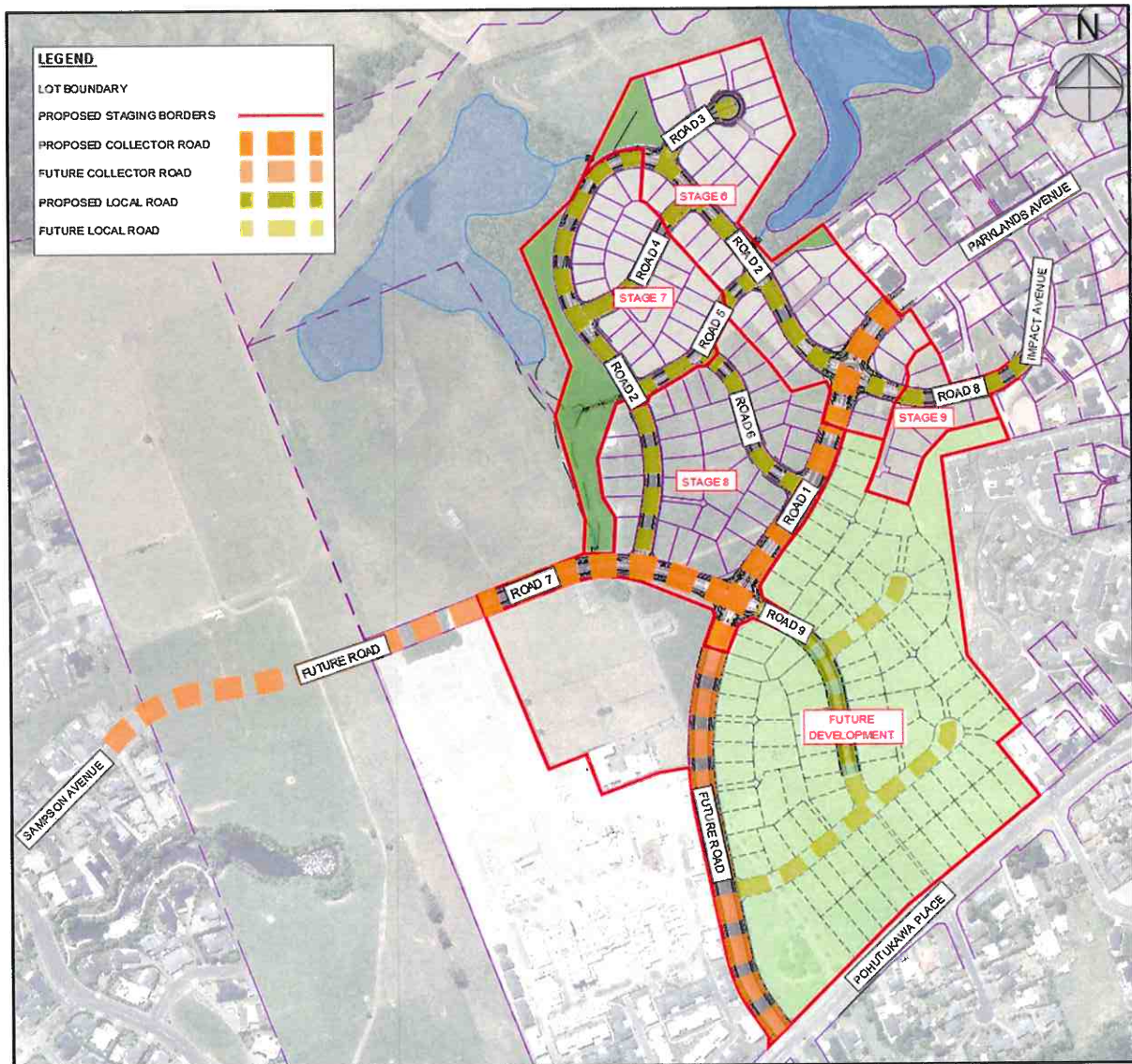
Figure 2 – Red Jacket Rooding Layout Plan
