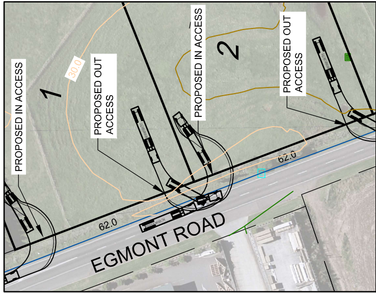
TURNING CIRCLES LOT 1 & 2 SEMI-TRAILER SCALE 1:1250
